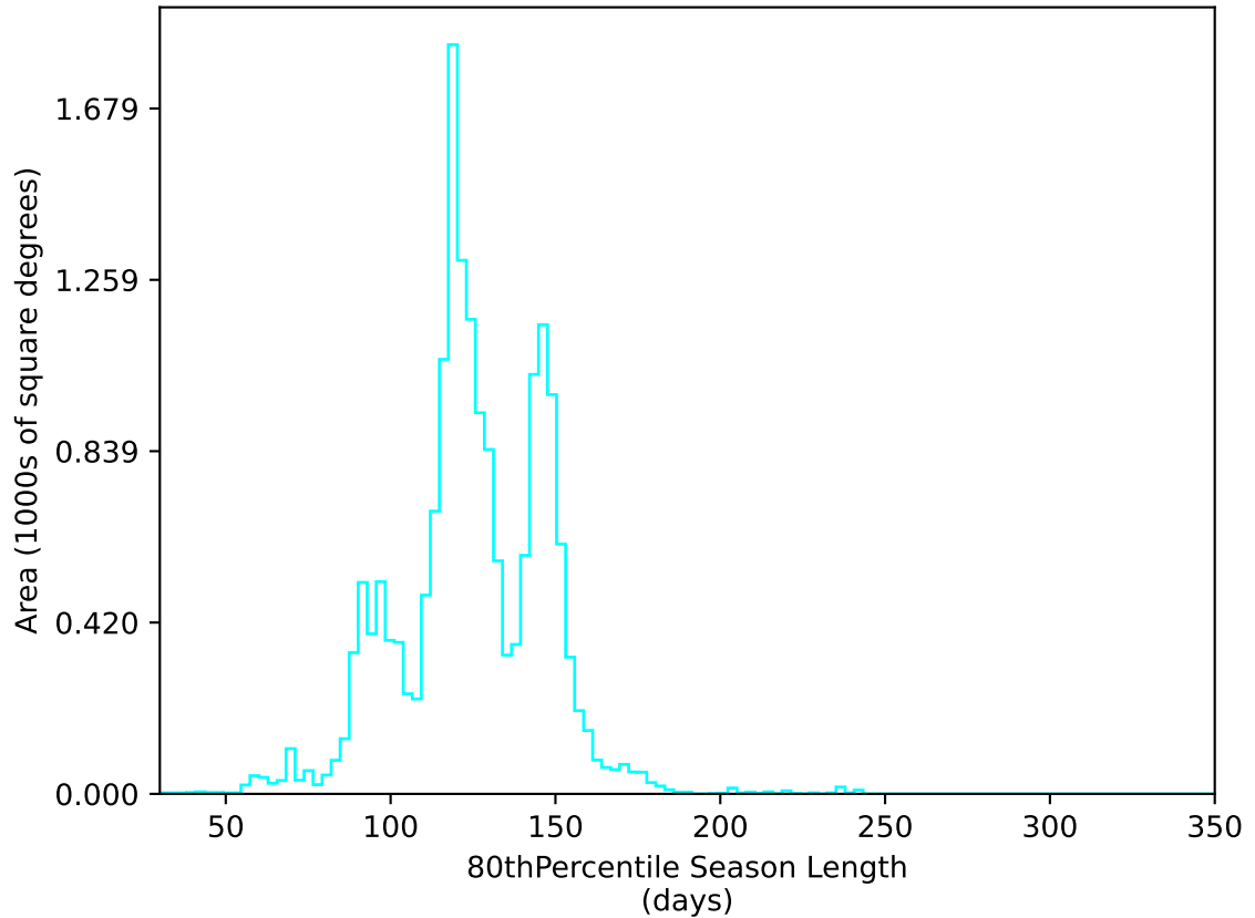
ddf_acor_sf10_lsf15_lsr20_v3.4_10yrs WFD u band: 80thPercentile Season Length
