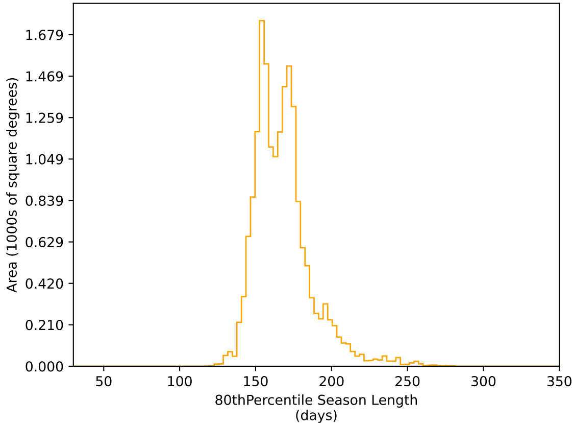
ddf_acor_sf10_lsf15_lsr20_v3.4_10yrs WFD r band: 80thPercentile Season Length
