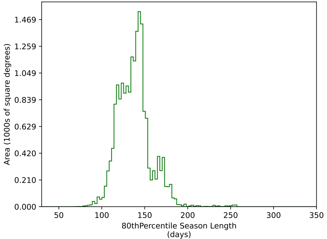
ddf_acor_sf10_lsf15_lsr20_v3.4_10yrs WFD g band: 80thPercentile Season Length
