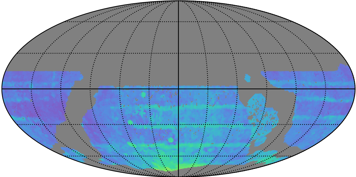
ddf_acor_sf10_lsf15_lsr20_v3.4_10yrs WFD all bands: 80thPercentile Season Length
