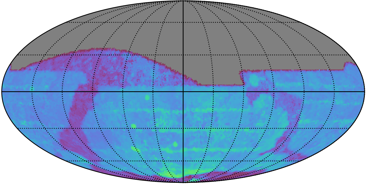
ddf_acor_sf10_lsf15_lsr20_v3.4_10yrs All sky z band: 80thPercentile Season Length
