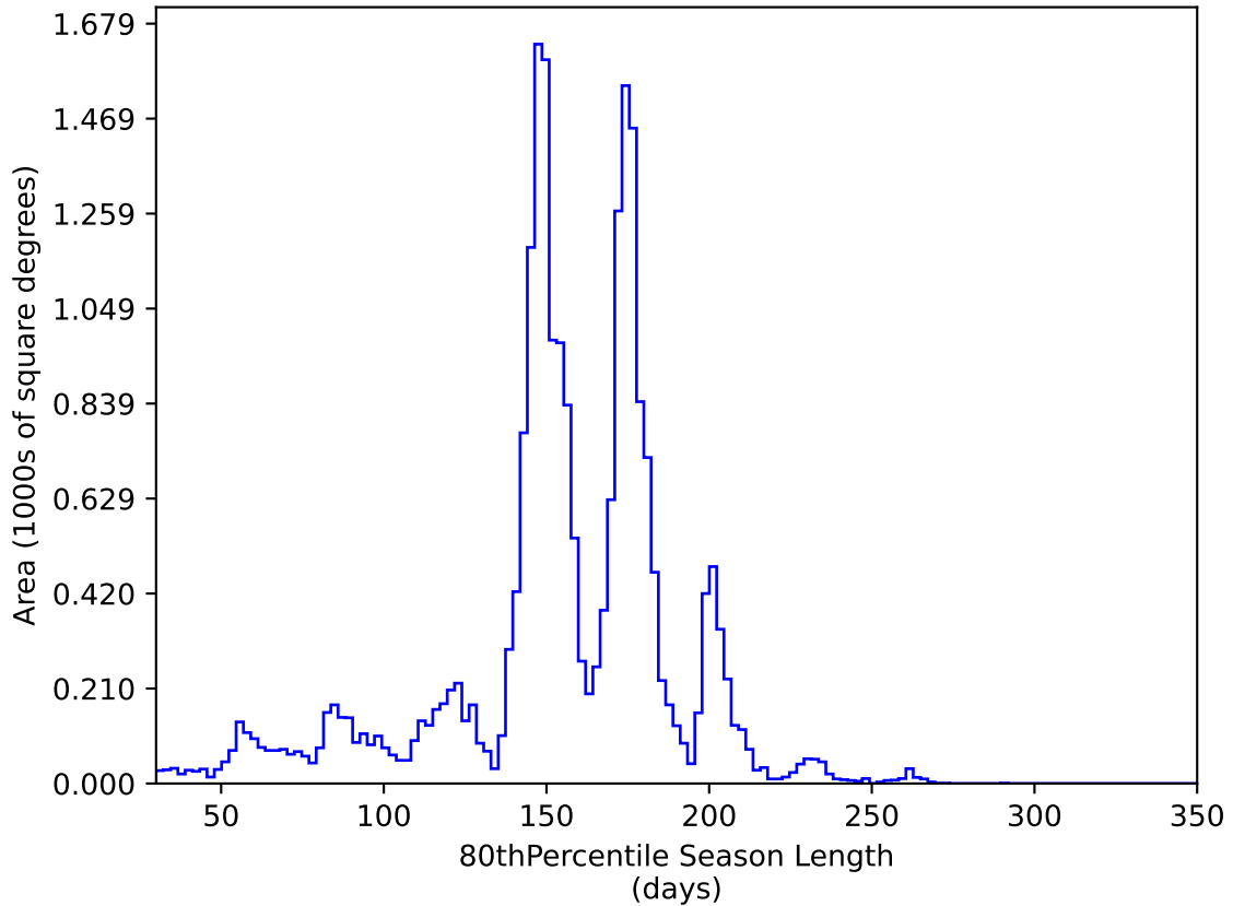
ddf_acor_sf10_ls15_lsr20_v3.4_10yrs All sky y band: 80thPercentile Season Length
