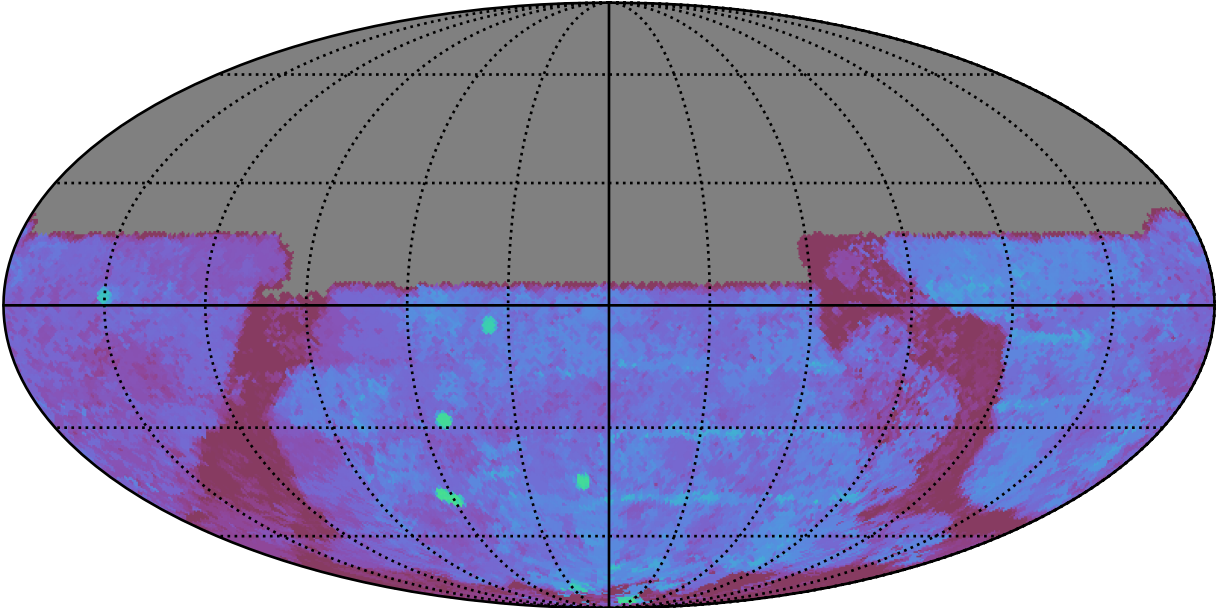
ddf_acor_sf10_lsf15_lsr20_v3.4_10yrs All sky u band: 80thPercentile Season Length
