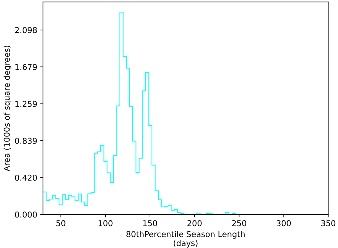
ddf_acor_sf10_lsf15_lsr20_v3.4_10yrs All sky u band: 80thPercentile Season Length
