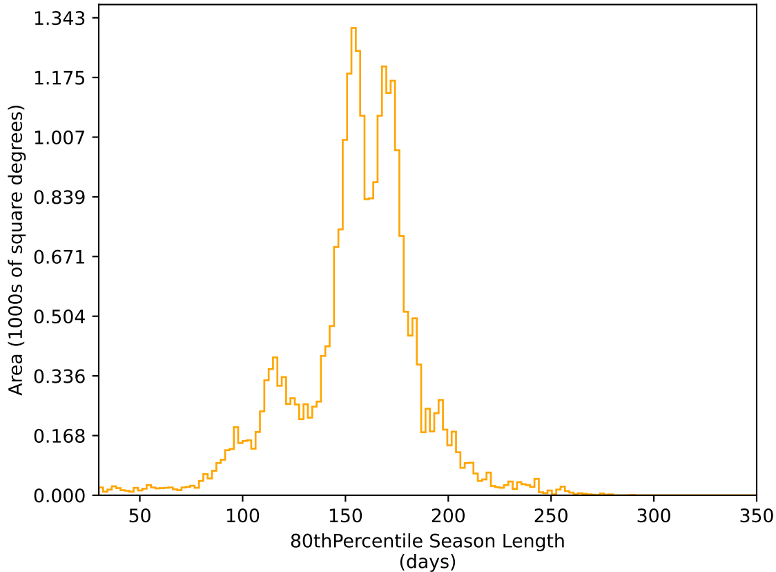
ddf_acor_sf10_lsf15_lsr20_v3.4_10yrs All sky r band: 80thPercentile Season Length
