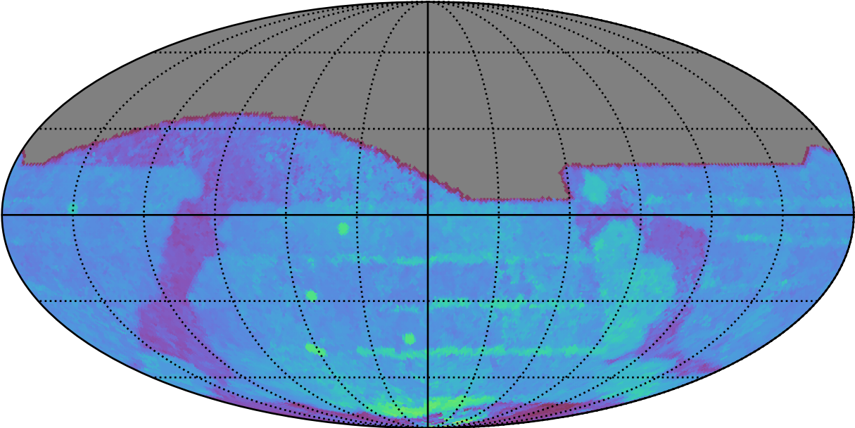
ddf_acor_sf10_lsf15_lsr20_v3.4_10yrs All sky i band: 80thPercentile Season Length
