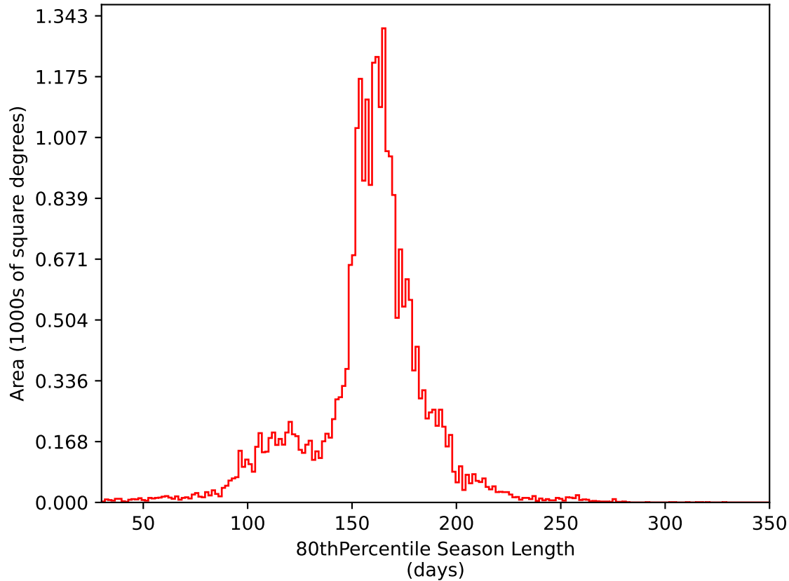
ddf_acor_sf10_lsf15_lsr20_v3.4_10yrs All sky i band: 80thPercentile Season Length
