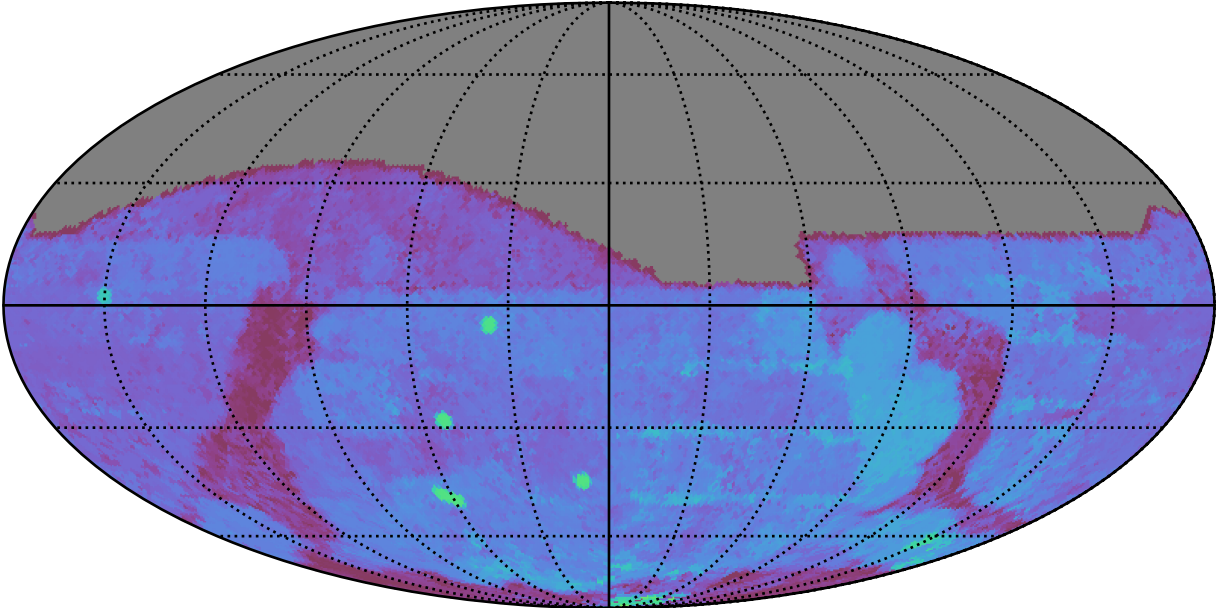
ddf_acor_sf10_lsf15_lsr20_v3.4_10yrs All sky g band: 80thPercentile Season Length
