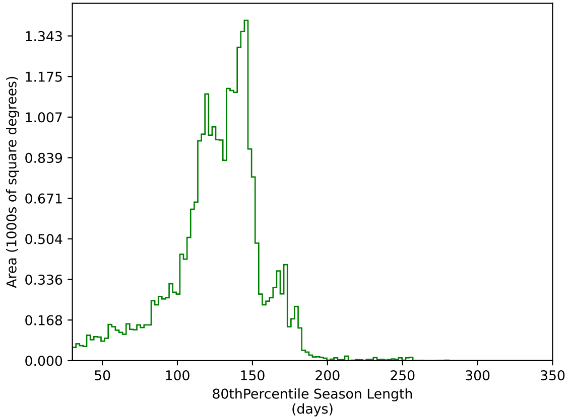
ddf_acor_sf10_lsf15_lsr20_v3.4_10yrs All sky g band: 80thPercentile Season Length
