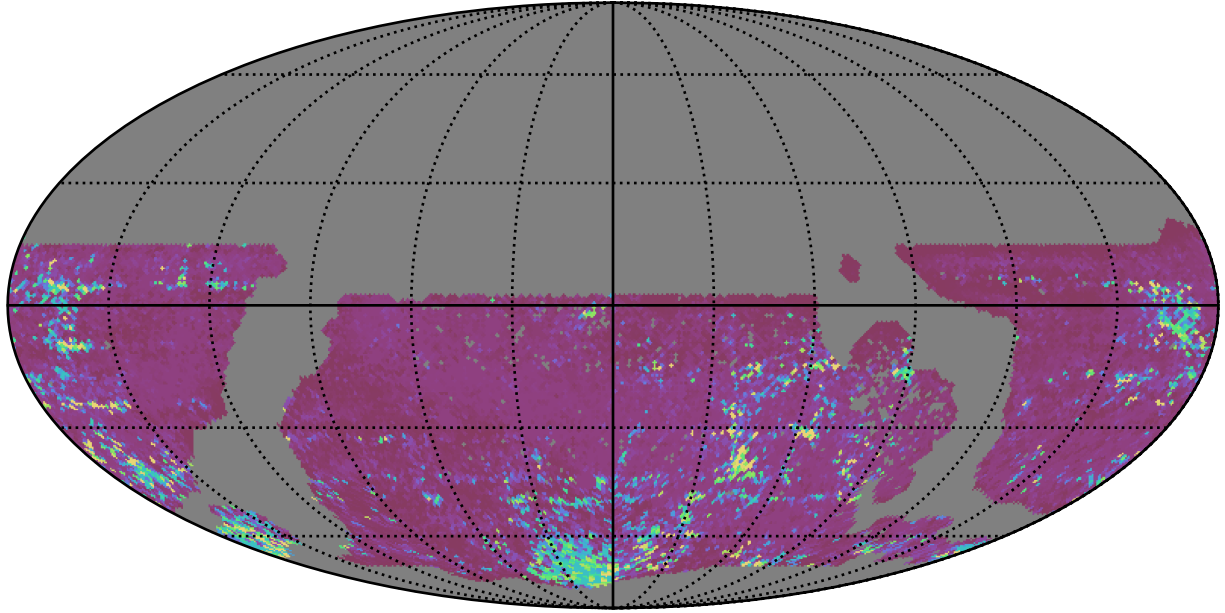
ddf_acor_sf10_lsf15_lsr20_v3.4_10yrs WFD z band: 75th Percentile Intranight Timespan
