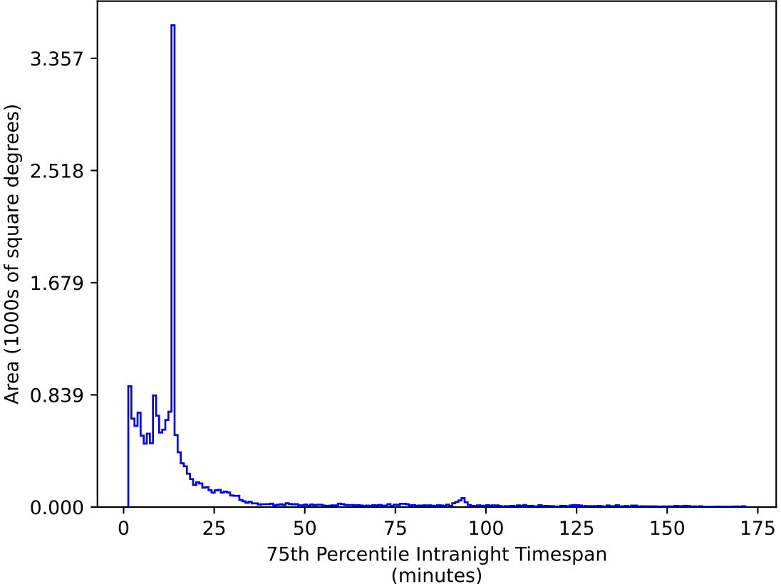
ddf_acor_sf10_lsf15_lsr20_v3.4_10yrs WFD z band: 75th Percentile Intranight Timespan
