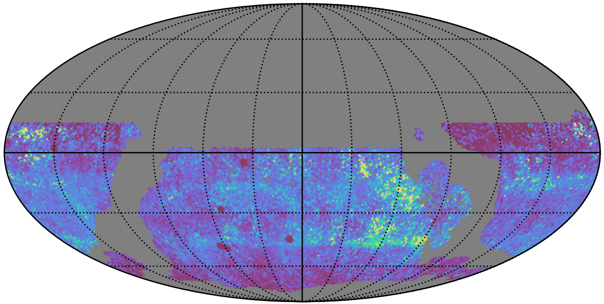
ddf_acor_sf10_lsf15_lsr20_v3.4_10yrs WFD y band: 75th Percentile Intranight Timespan
