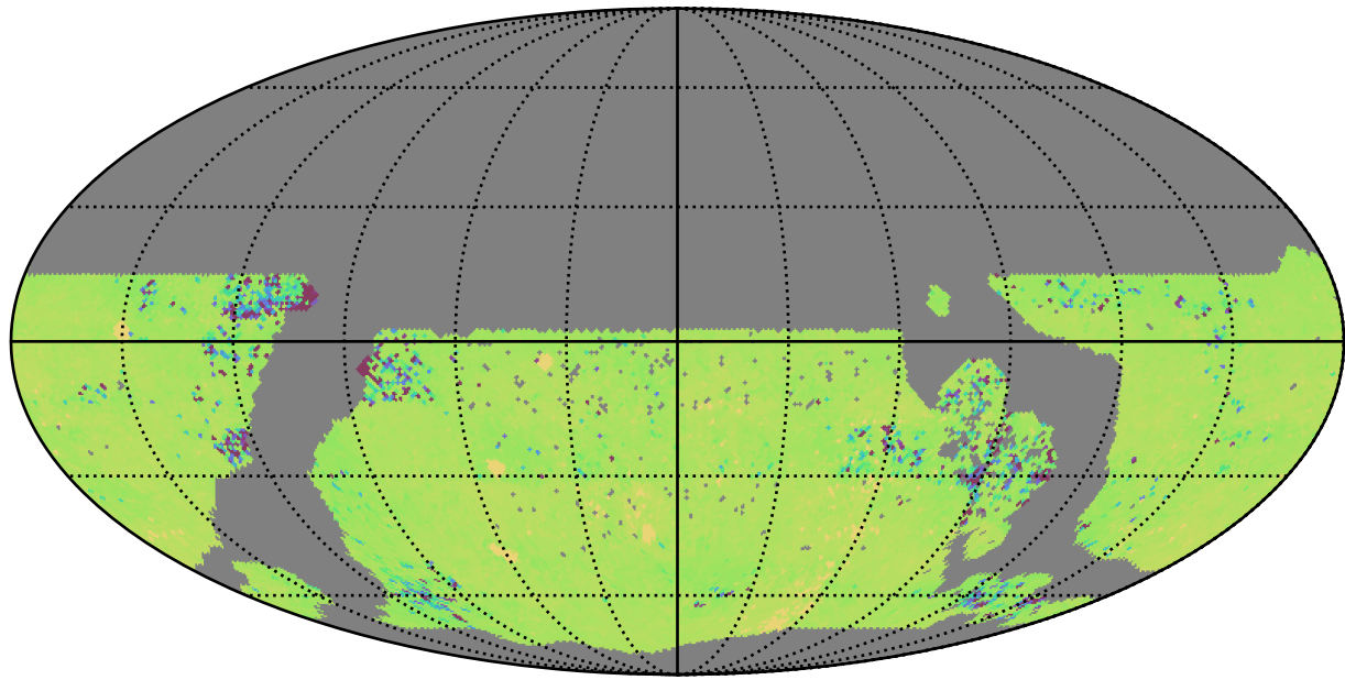
ddf_acor_sf10_lsf15_lsr20_v3.4_10yrs WFD ug bands: 75th Percentile Intranight Timespan
