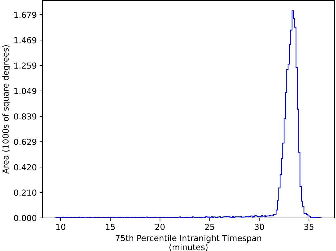
ddf_acor_sf10_lsf15_lsr20_v3.4_10yrs WFD ug bands: 75th Percentile Intranight Timespan
