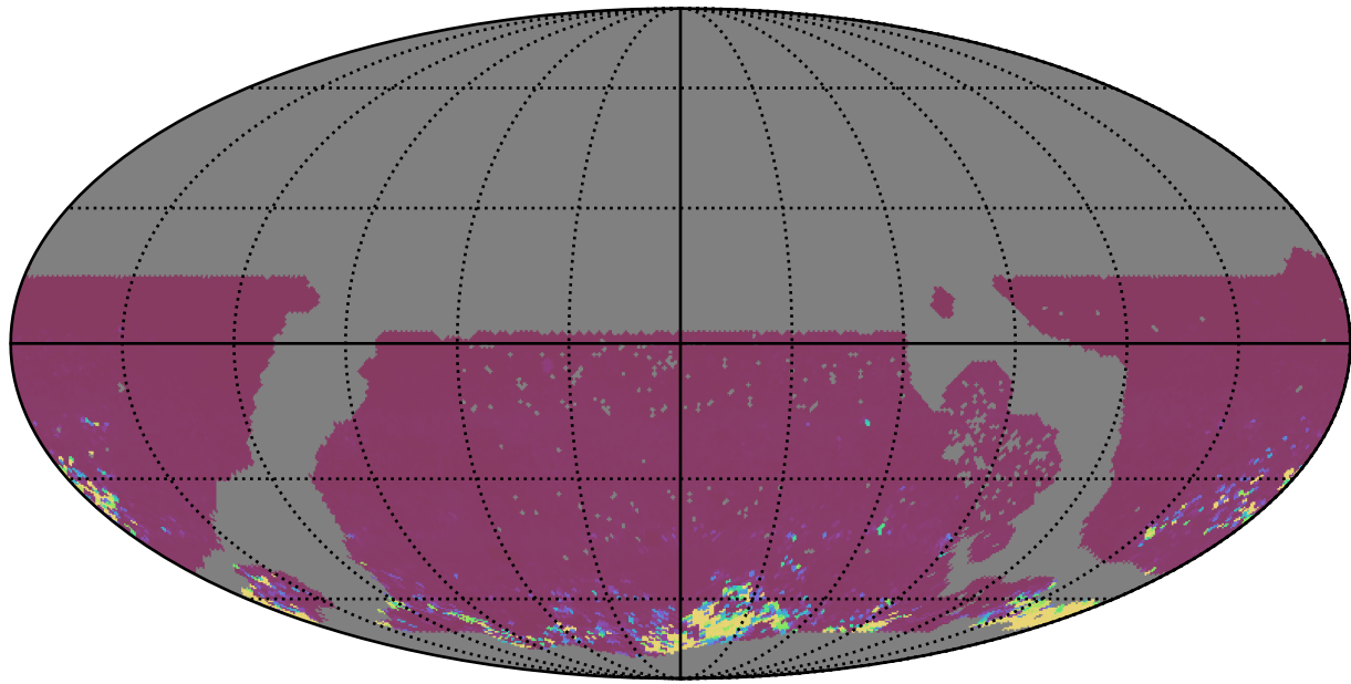
ddf_acor_sf10_ls15_lsr20_v3.4_10yrs WFD ri bands: 75th Percentile Intranight Timespan
