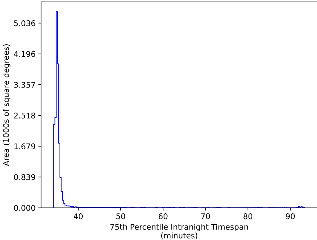
ddf_acor_sf10_ls15_lsr20_v3.4_10yrs WFD ri bands: 75th Percentile Intranight Timespan
