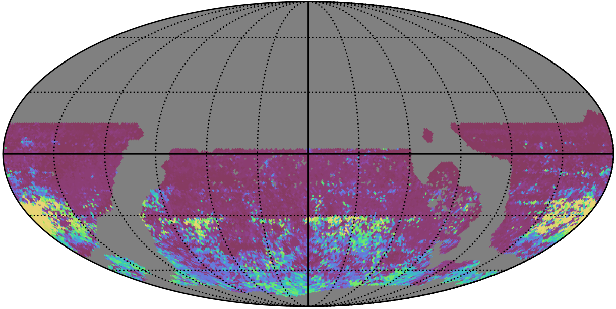
ddf_acor_sf10_ls15_lsr20_v3.4_10yrs WFD r band: 75th Percentile Intranight Timespan
