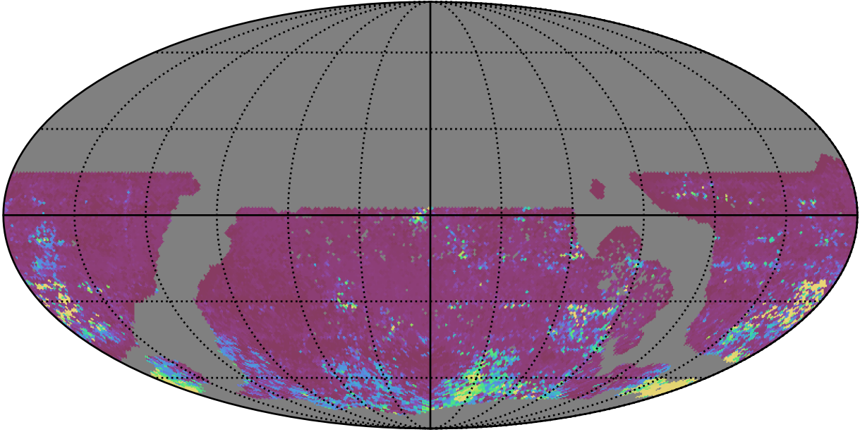
ddf_acor_sf10_lsf15_lsr20_v3.4_10yrs WFD i band: 75th Percentile Intranight Timespan
