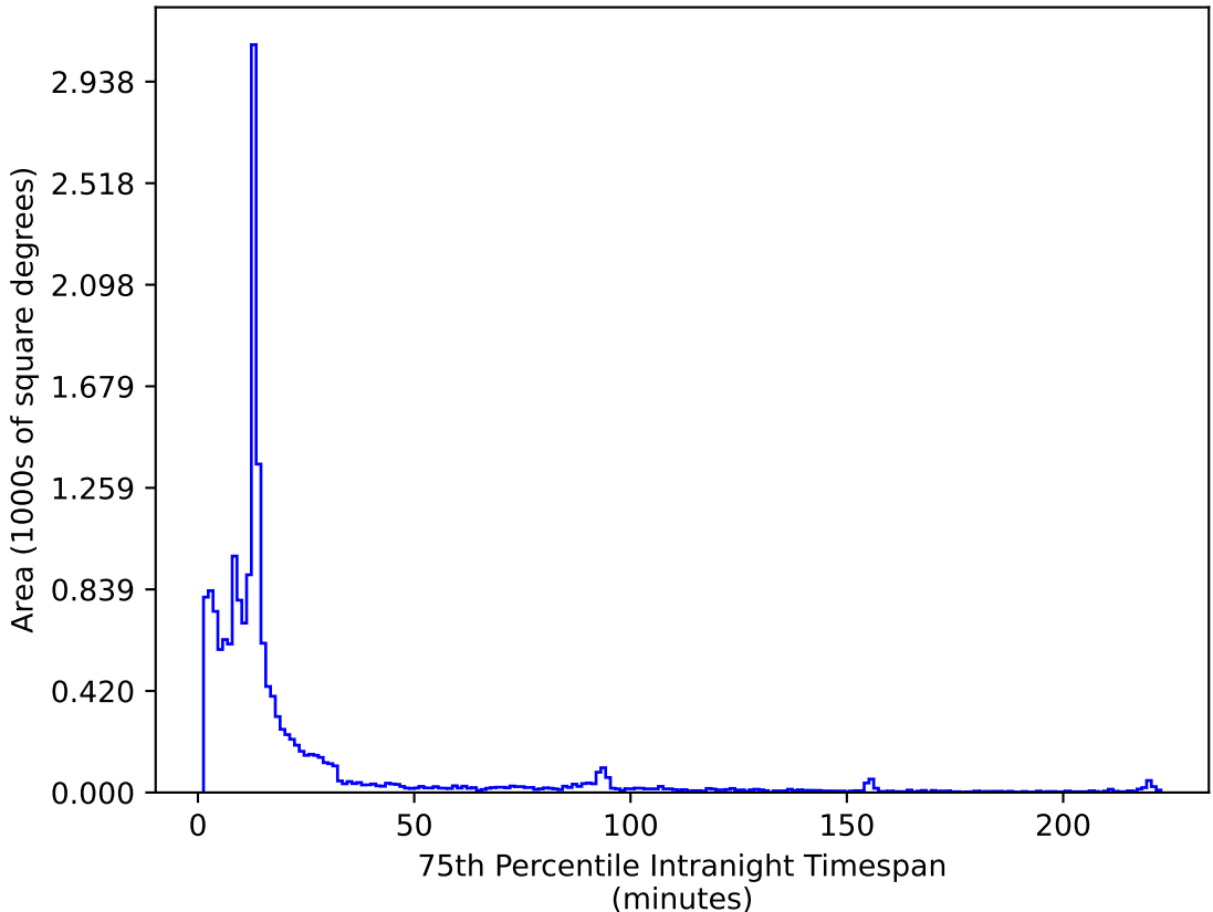
ddf_acor_sf10_ls15_lsr20_v3.4_10yrs WFD i band: 75th Percentile Intranight Timespan
