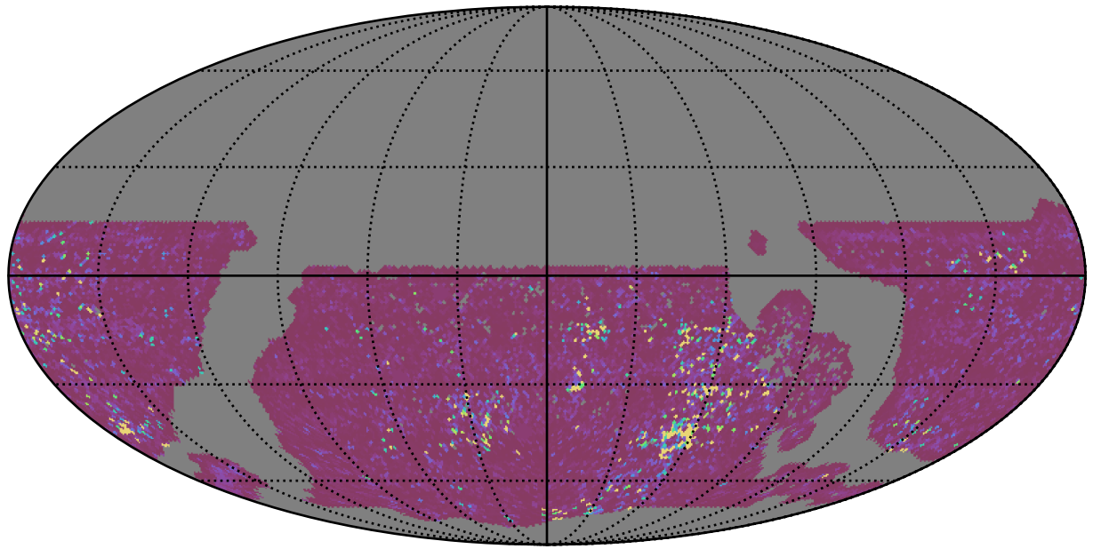
ddf_acor_sf10_lsf15_lsr20_v3.4_10yrs WFD g band: 75th Percentile Intranight Timespan
