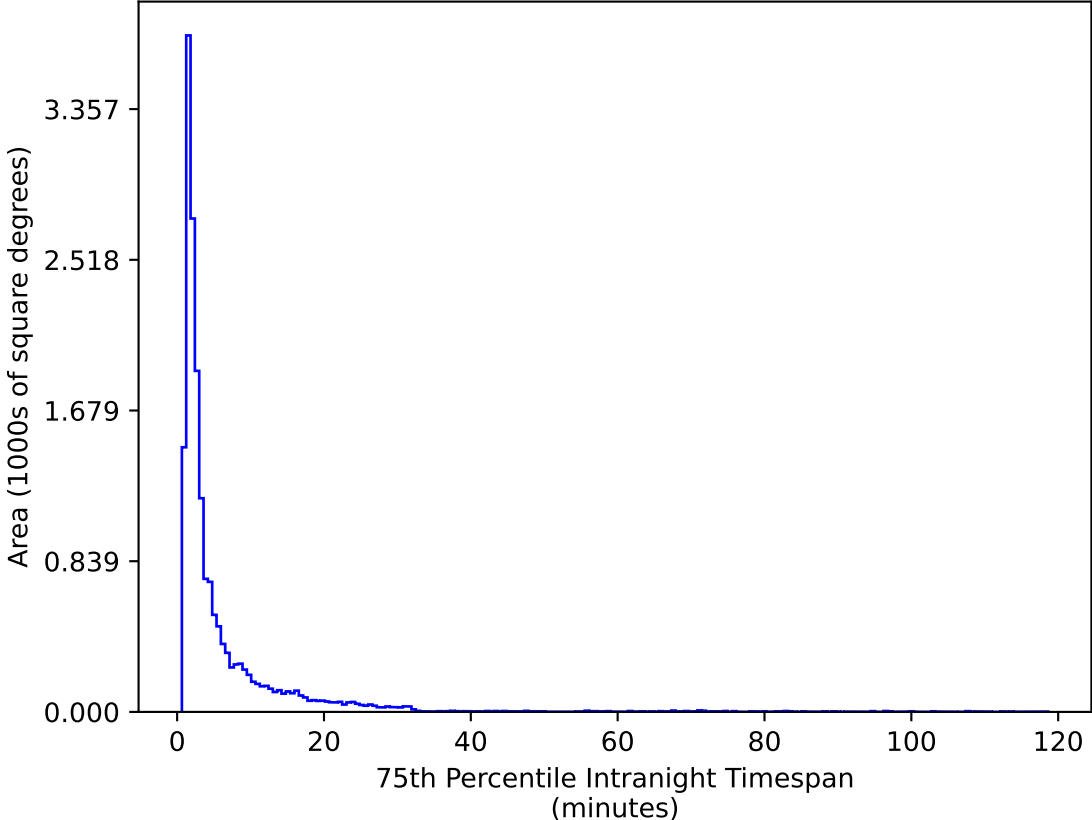
ddf_acor_sf10_lsf15_lsr20_v3.4_10yrs WFD g band: 75th Percentile Intranight Timespan
