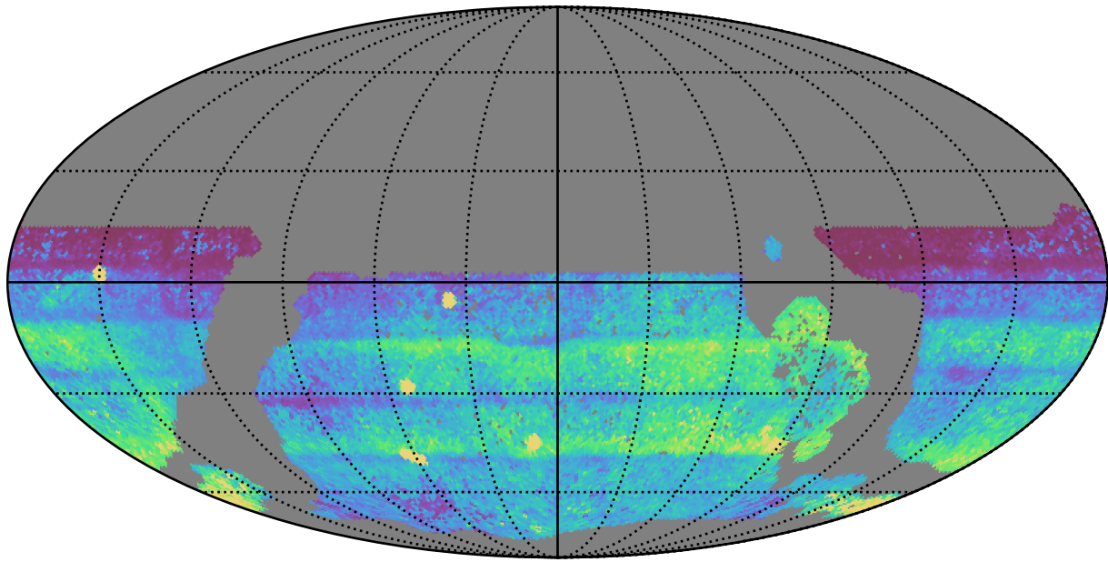
ddf_acor_sf10_lsf15_lsr20_v3.4_10yrs WFD all bands: 75th Percentile Intranight Timespan
