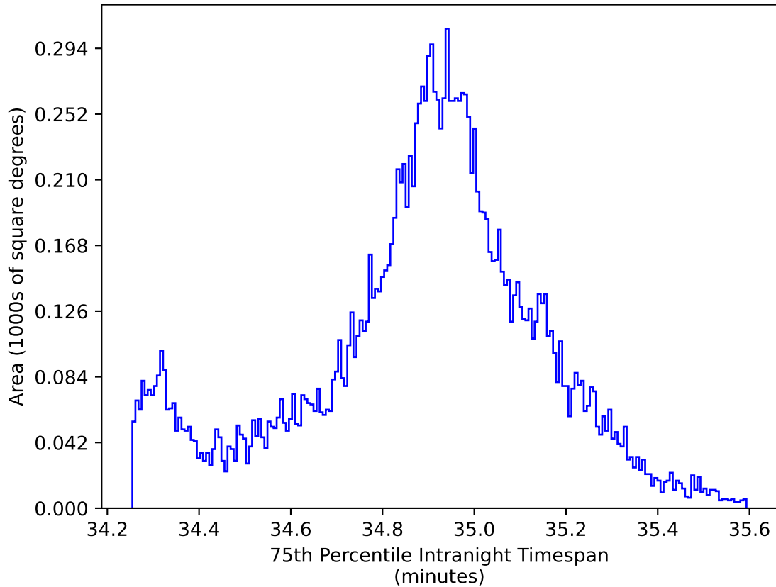
ddf_acor_sf10_lsf15_lsr20_v3.4_10yrs WFD all bands: 75th Percentile Intranight Timespan
