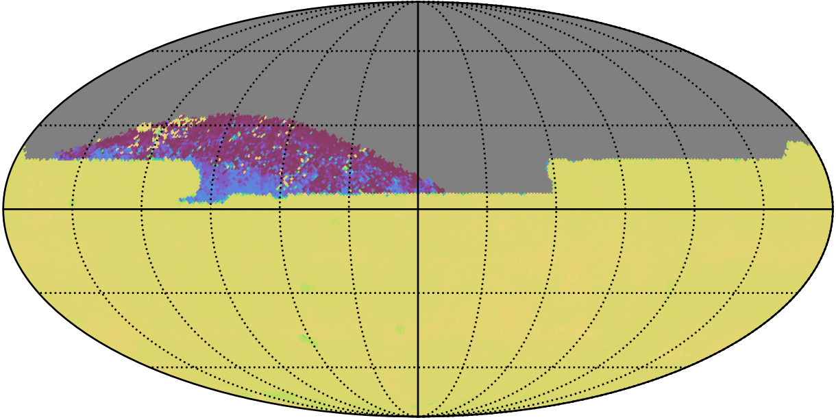
ddf_acor_sf10_lsf15_lsr20_v3.4_10yrs All sky zy bands: 75th Percentile Intranight Timespan
