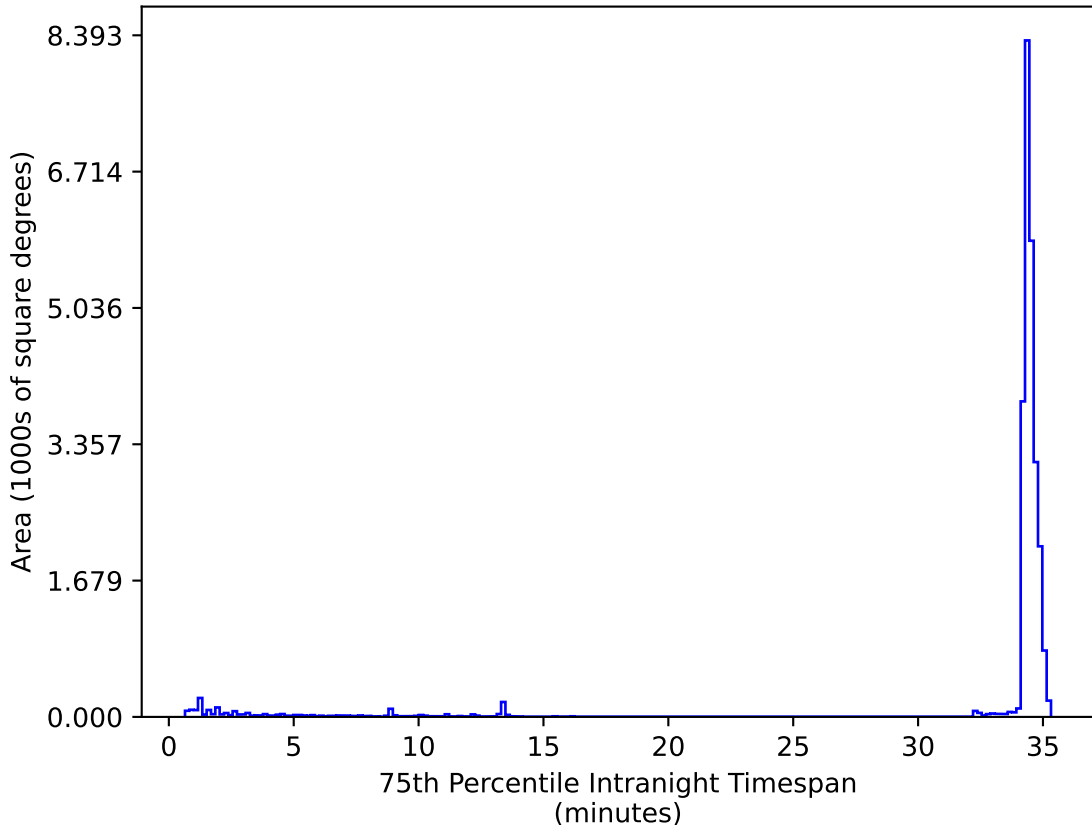
ddf_acor_sf10_lsf15_lsr20_v3.4_10yrs All sky zy bands: 75th Percentile Intranight Timespan
