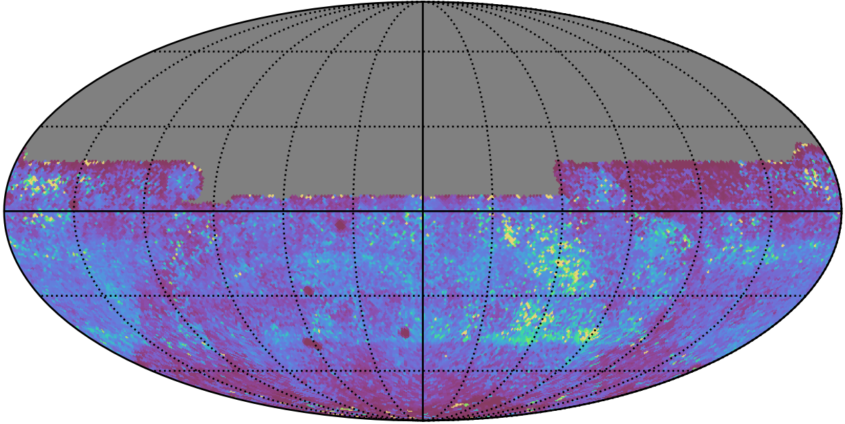
ddf_acor_sf10_lsf15_lsr20_v3.4_10yrs All sky y band: 75th Percentile Intranight Timespan
