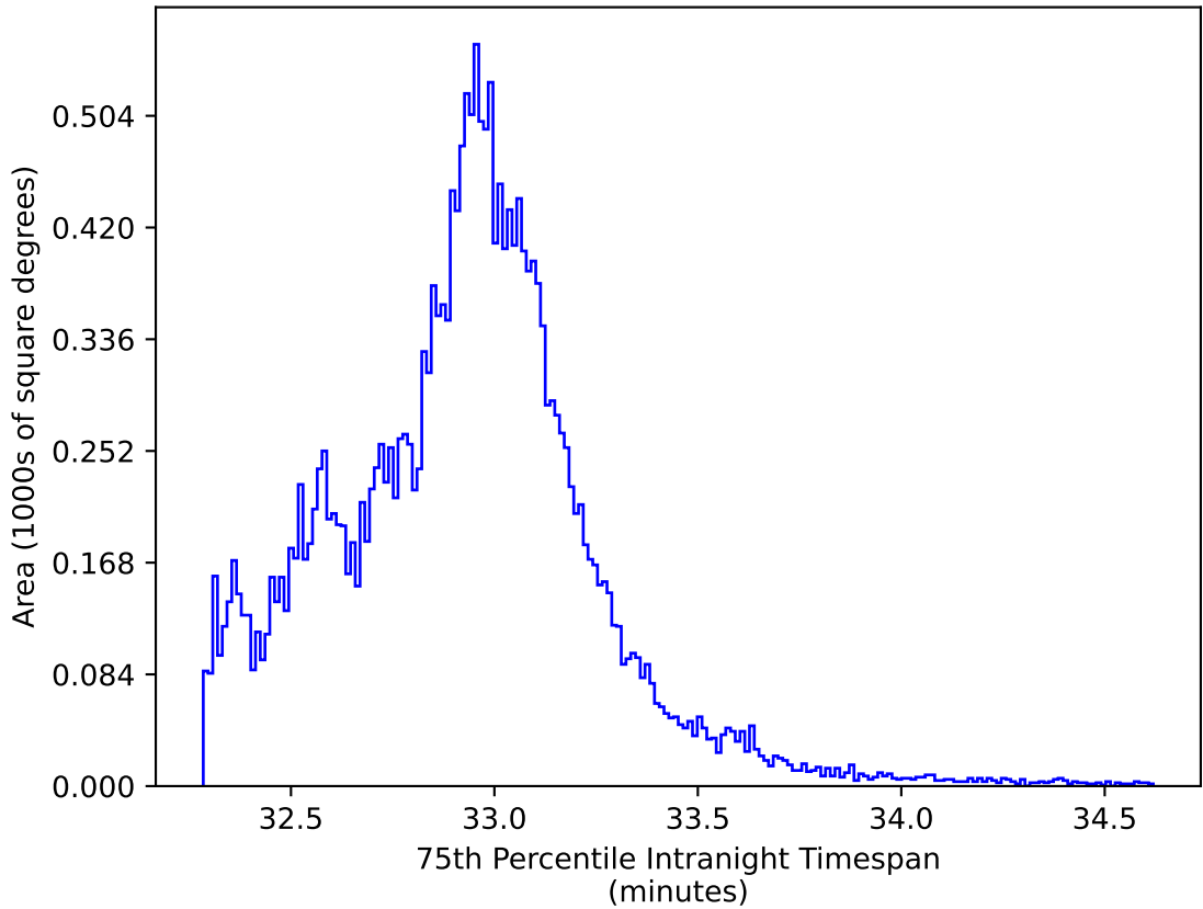
ddf_acor_sf10_lsf15_lsr20_v3.4_10yrs All sky y band: 75th Percentile Intranight Timespan
