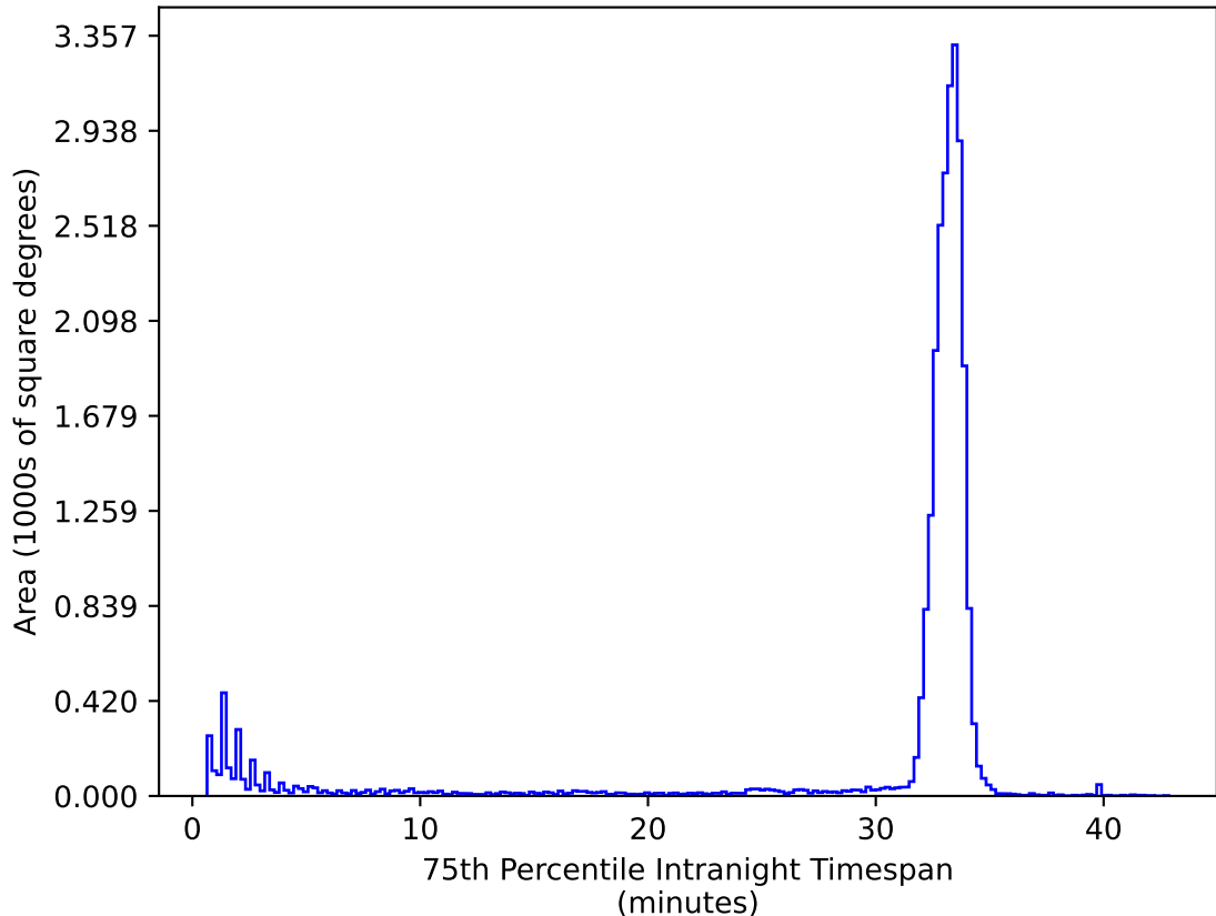
ddf_acor_sf10_lsf15_lsr20_v3.4_10yrs All sky ug bands: 75th Percentile Intranight Timespan
