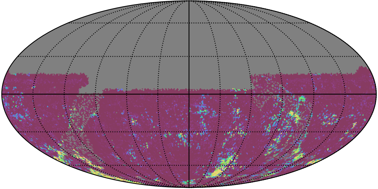
ddf_acor_sf10_lsf15_lsr20_v3.4_10yrs All sky u band: 75th Percentile Intranight Timespan
