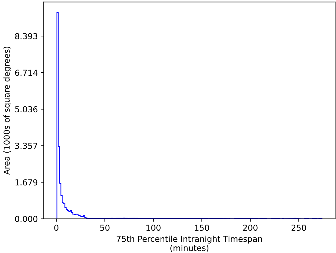
ddf_acor_sf10_lsf15_lsr20_v3.4_10yrs All sky u band: 75th Percentile Intranight Timespan
