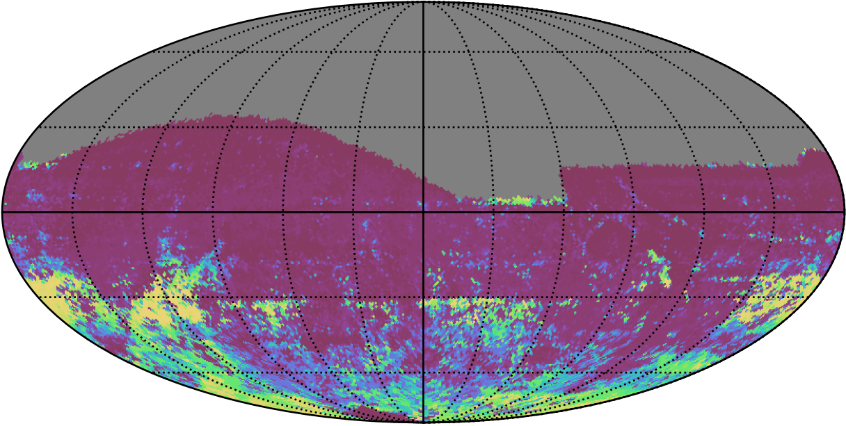
ddf_acor_sf10_lsf15_lsr20_v3.4_10yrs All sky r band: 75th Percentile Intranight Timespan
