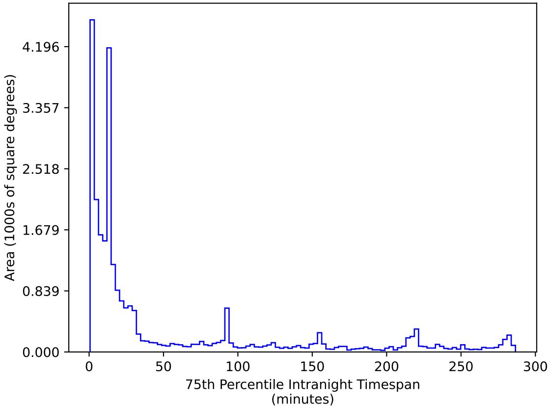
ddf_acor_sf10_ls15_lsr20_v3.4_10yrs All sky r band: 75th Percentile Intranight Timespan
