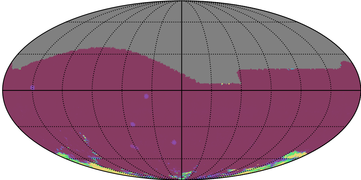
ddf_acor_sf10_lsf15_lsr20_v3.4_10yrs All sky iz bands: 75th Percentile Intranight Timespan
