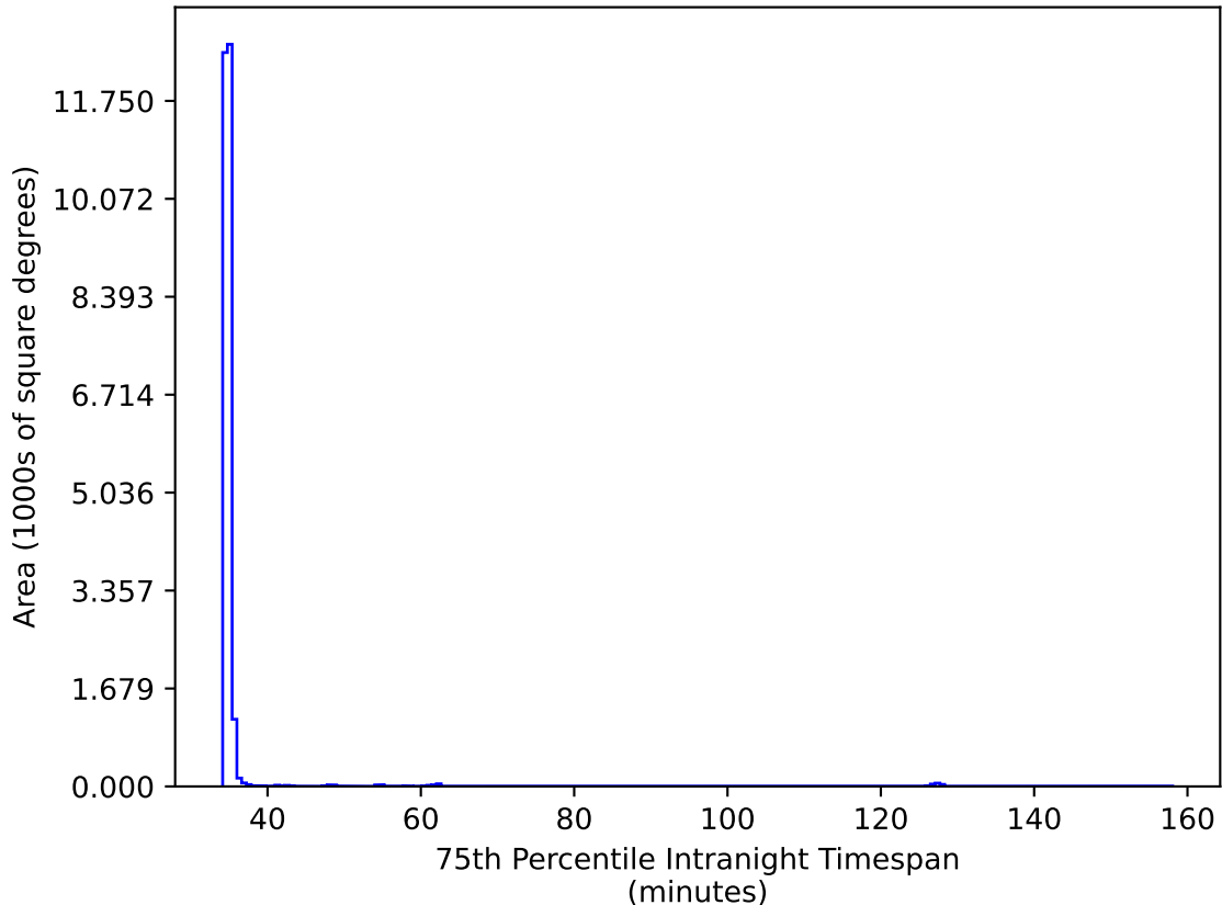
ddf_acor_sf10_ls15_lsr20_v3.4_10yrs All sky iz bands: 75th Percentile Intranight Timespan
