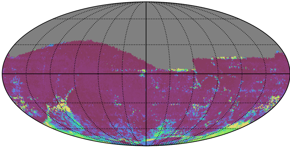
ddf_acor_sf10_lsf15_lsr20_v3.4_10yrs All sky i band: 75th Percentile Intranight Timespan
