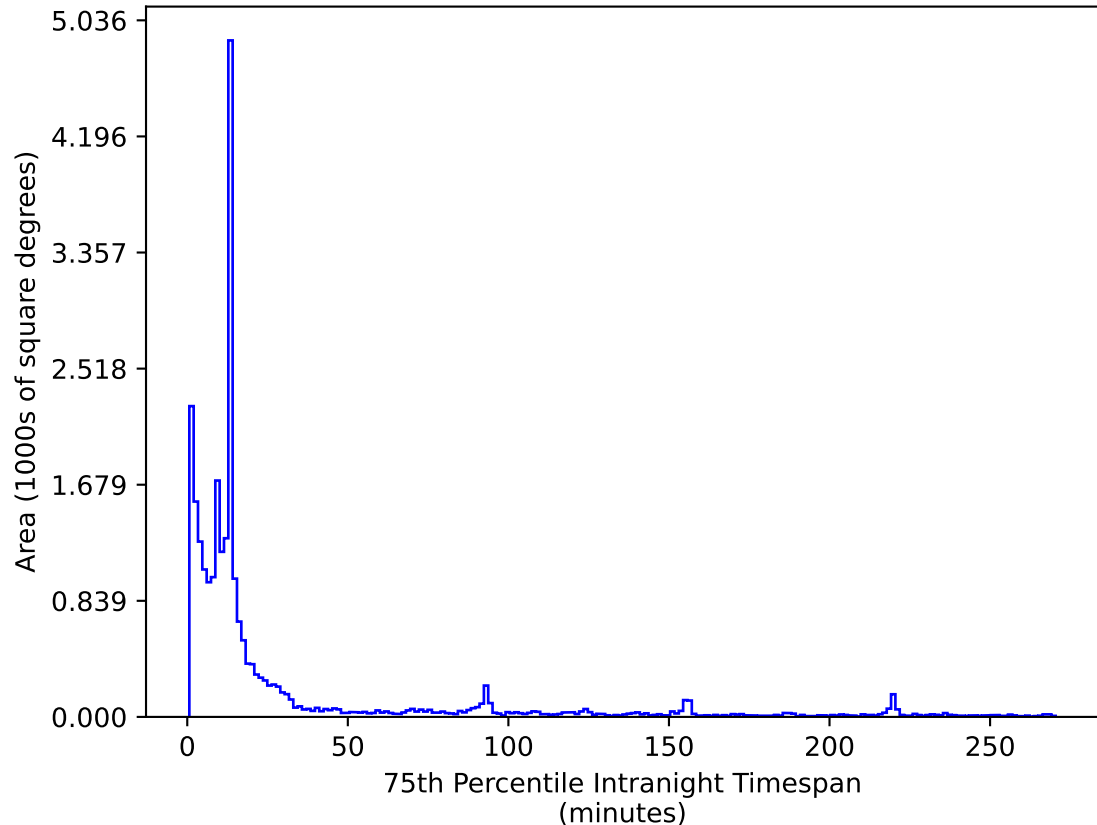
ddf_acor_sf10_ls15_lsr20_v3.4_10yrs All sky i band: 75th Percentile Intranight Timespan
