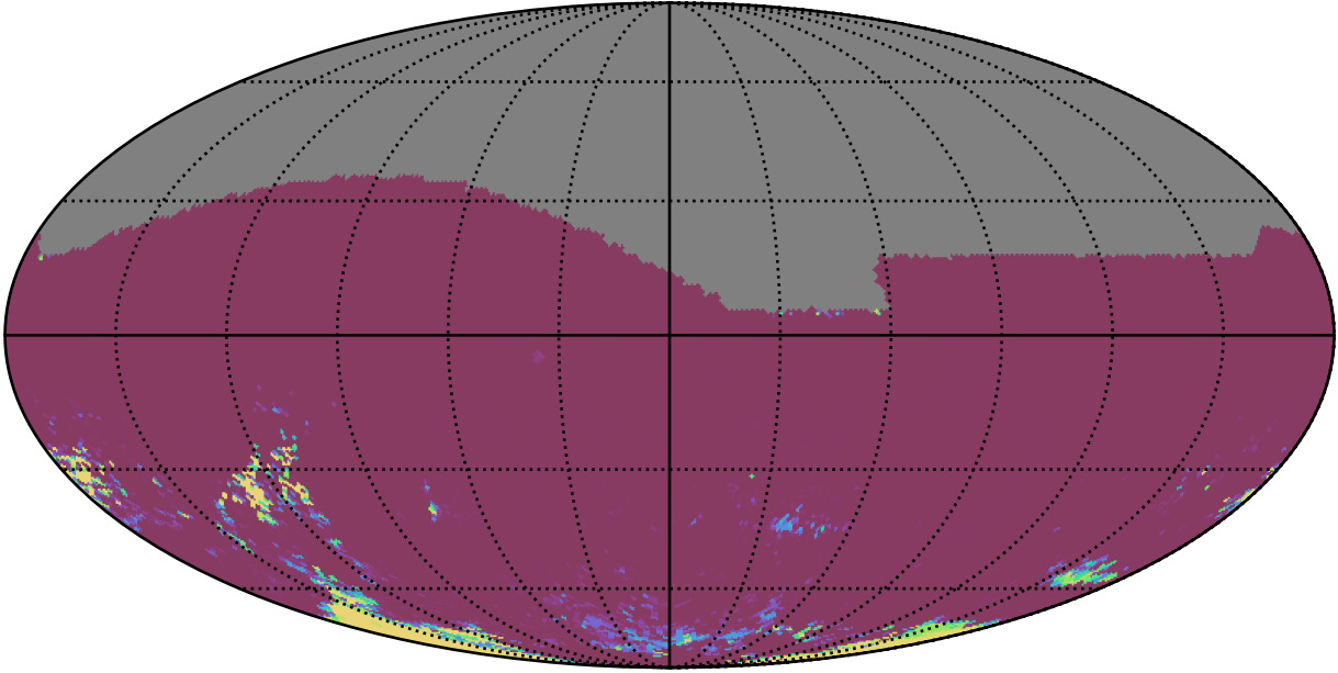
ddf_acor_sf10_lsf15_lsr20_v3.4_10yrs All sky gr bands: 75th Percentile Intranight Timespan
