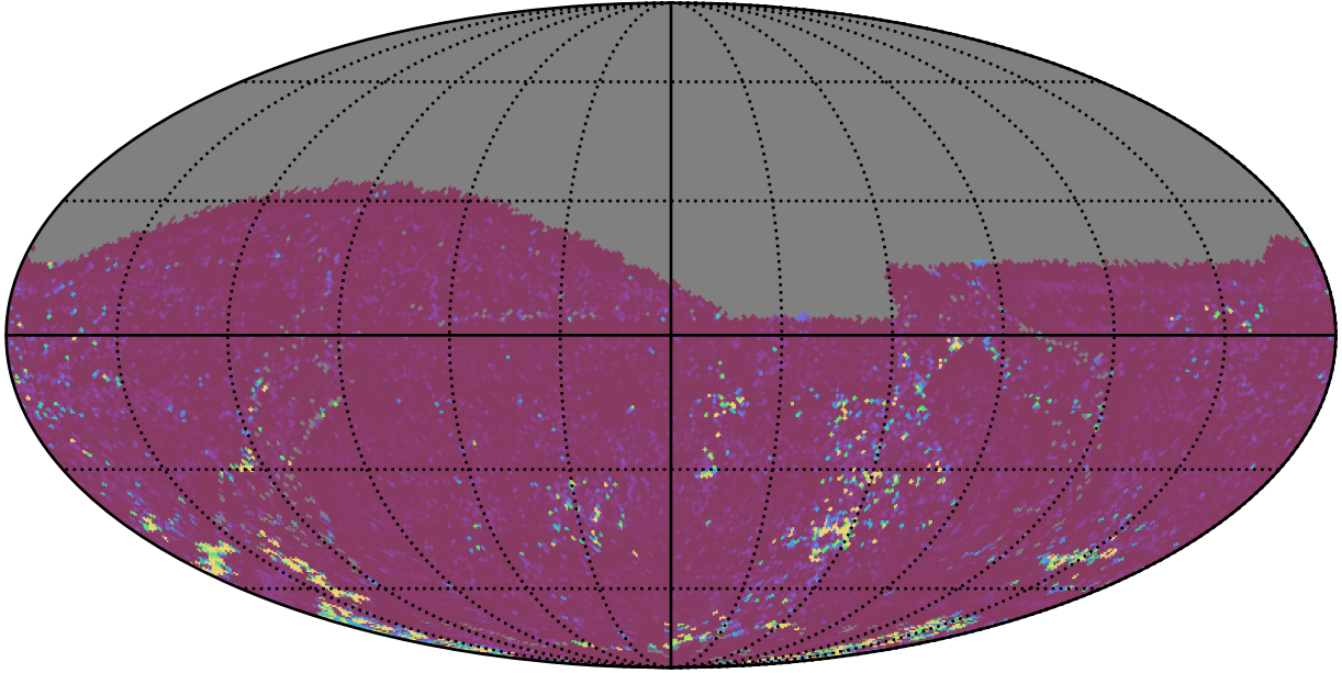
ddf_acor_sf10_lsf15_lsr20_v3.4_10yrs All sky g band: 75th Percentile Intranight Timespan
