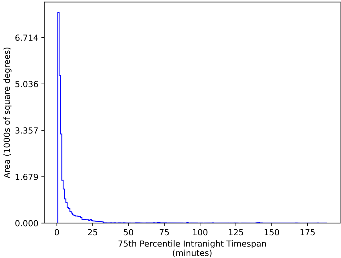
ddf_acor_sf10_lsf15_lsr20_v3.4_10yrs All sky g band: 75th Percentile Intranight Timespan
