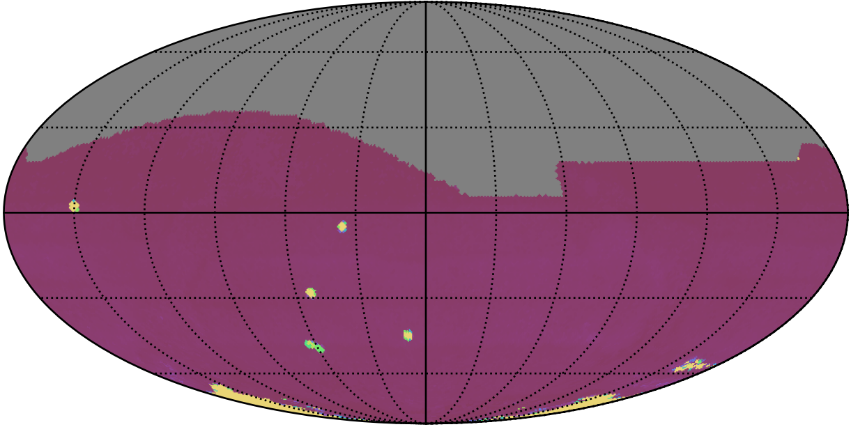
ddf_acor_sf10_lsf15_lsr20_v3.4_10yrs All sky all bands: 75th Percentile Intranight Timespan
