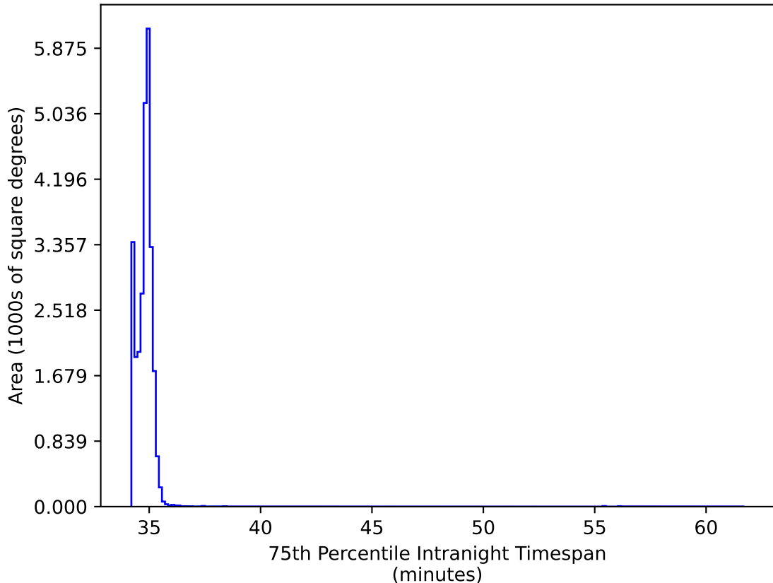
ddf_acor_sf10_lsf15_lsr20_v3.4_10yrs All sky all bands: 75th Percentile Intranight Timespan
