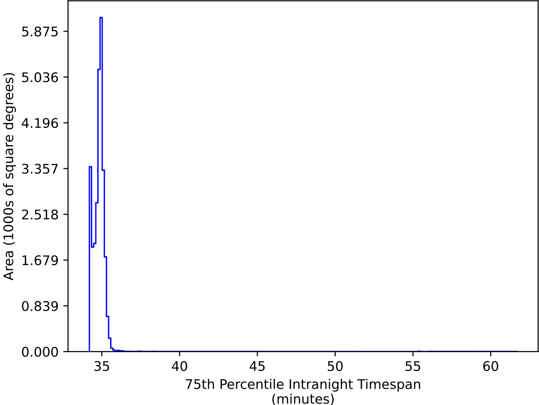
ddf_acor_sf10_lsf15_lsr20_v3.4_10yrs All sky: 75th Percentile Intranight Timespan
