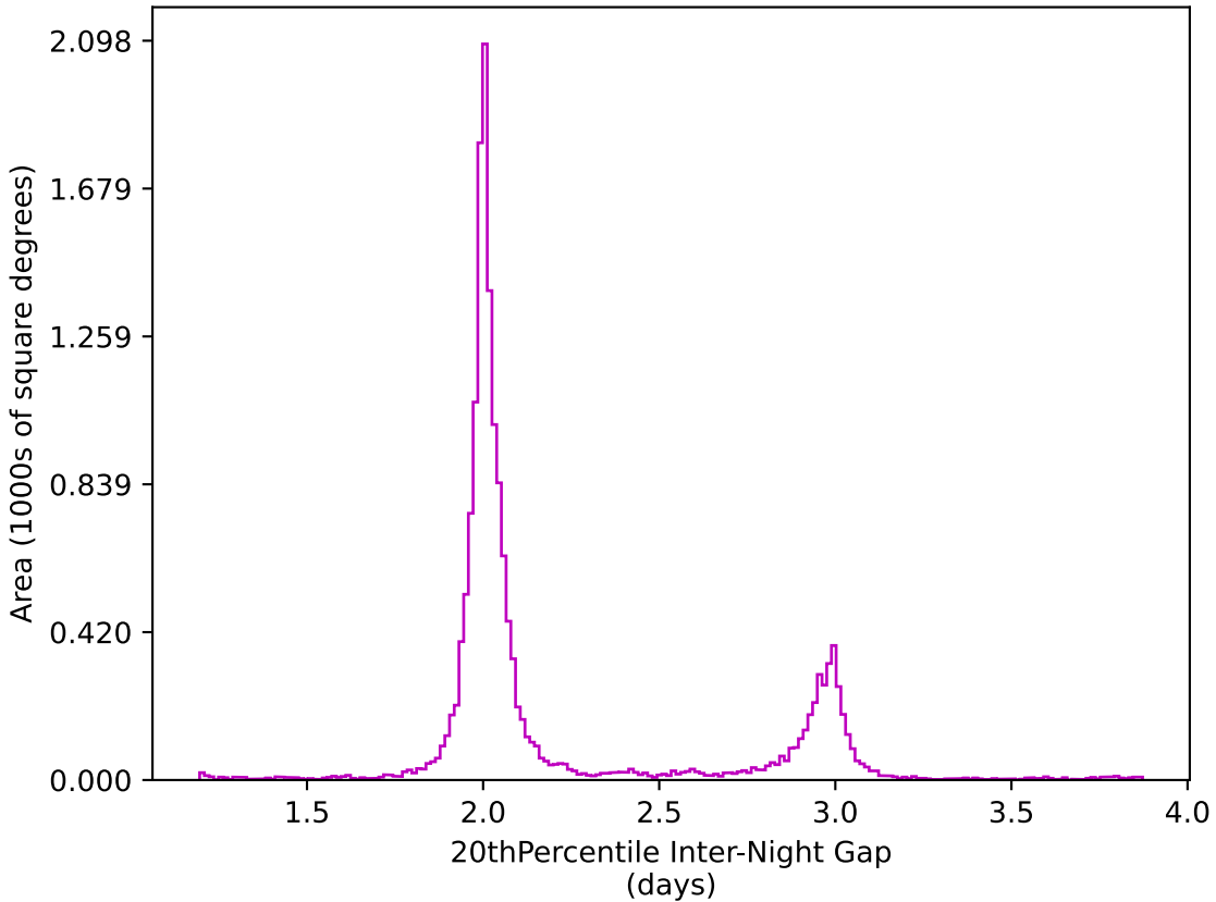
ddf_acor_sf10_lsf15_lsr20_v3.4_10yrs WFD z band: 20thPercentile Inter-Night Gap
