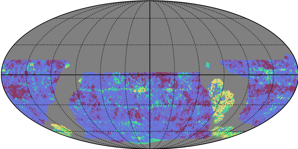
ddf_acor_sf10_lsf15_lsr20_v3.4_10yrs WFD y band: 20thPercentile Inter-Night Gap
