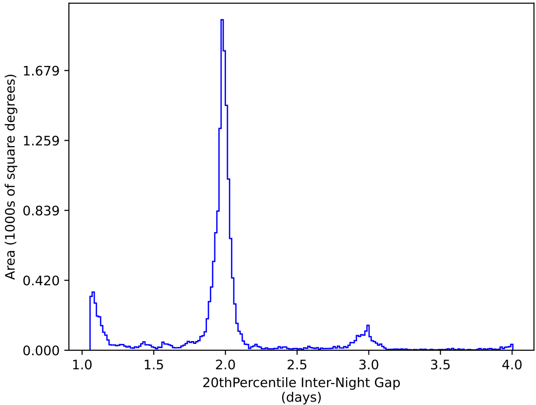
ddf_acor_sf10_ls15_lsr20_v3.4_10yrs WFD y band: 20thPercentile Inter-Night Gap
