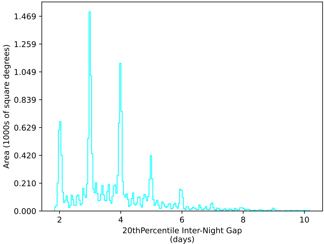
ddf_acor_sf10_ls15_lsr20_v3.4_10yrs WFD u band: 20thPercentile Inter-Night Gap
